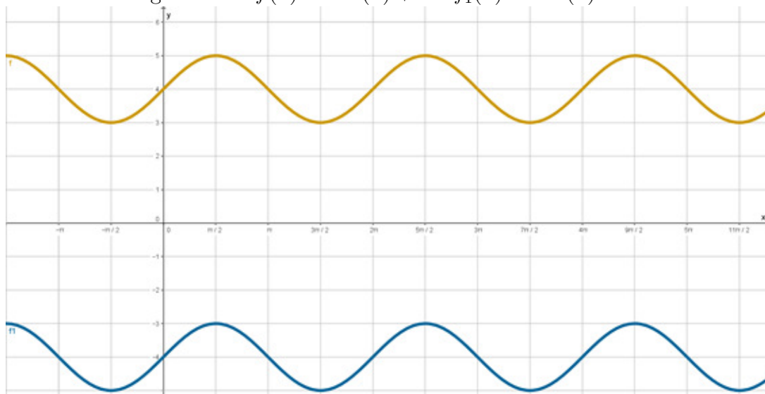
Figura 5.12: f(x) = \text{sen}(x) + 4 e f_1(x) = \text{sen}(x) - 4 .
