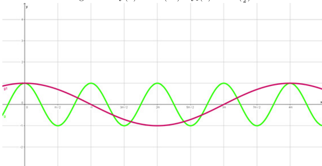
Figura 5.7: f(x) = \text{sen}(2x) e f_1(x) = \text{sen}(\frac{x}{2}) .
