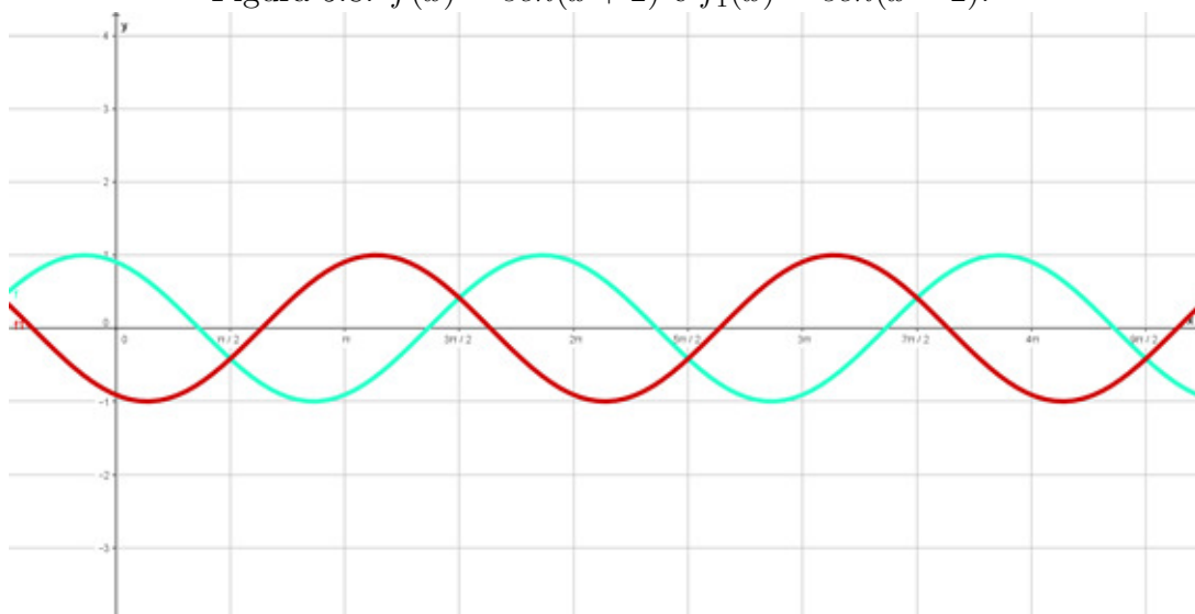
Figura 5.8: f(x) = \text{sen}(x + 2) e f_1(x) = \text{sen}(x - 2) .
